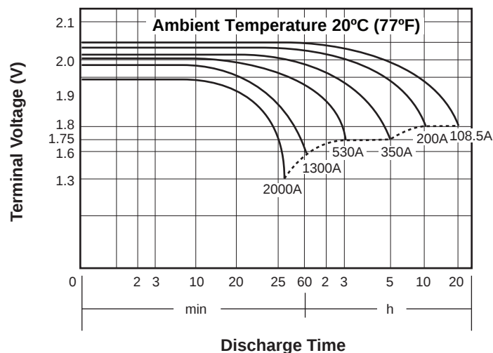
Discharge Characteristics
